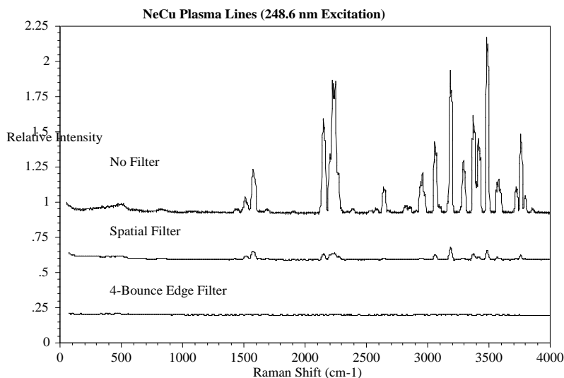
Typical laser line filter application.
