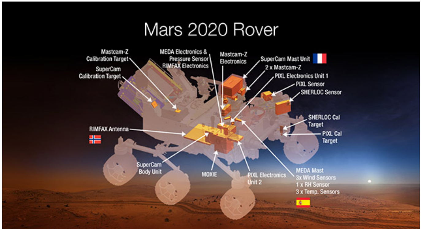
This diagram shows components of the investigations payload for NASA's Mars 2020 rover mission. Image credit: NASA/JPL-Caltech
